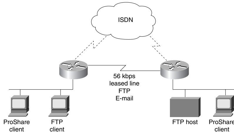
Figure 13-21 Policy-based routing.
