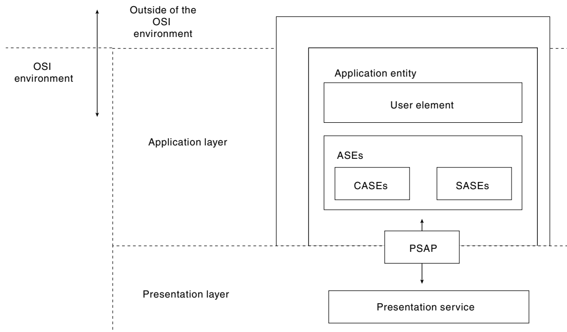
Figure 30-5 An Application Process Relies on the PSAP and Presentation Service
